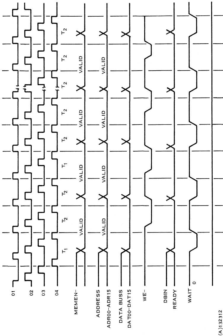
Figure E-2. 9900 Bus Write Cycle
