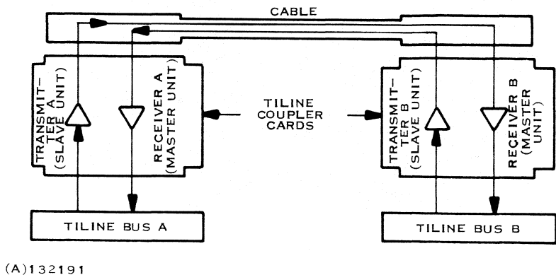
Figure 2-8. The TILINE Link
