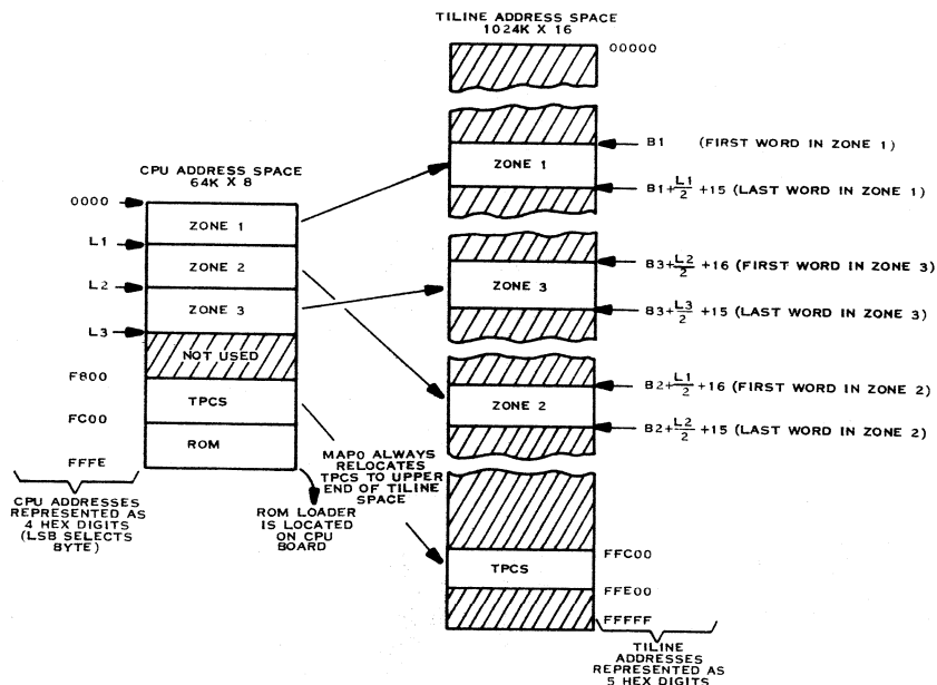
Figure 2-13. 990/10 CPU-TILINE Address Space with Map Option
