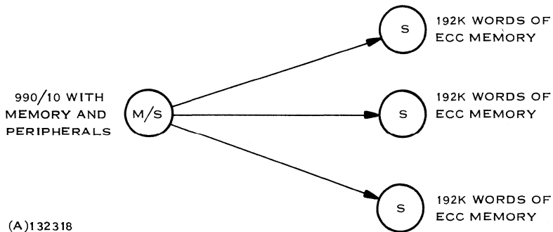
Figure F-5. Some Useful TILINE Configurations
