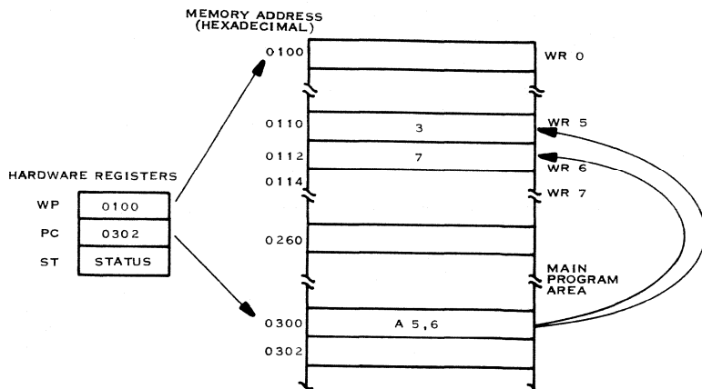
Figure 3-5. Workspace Register Addressing
