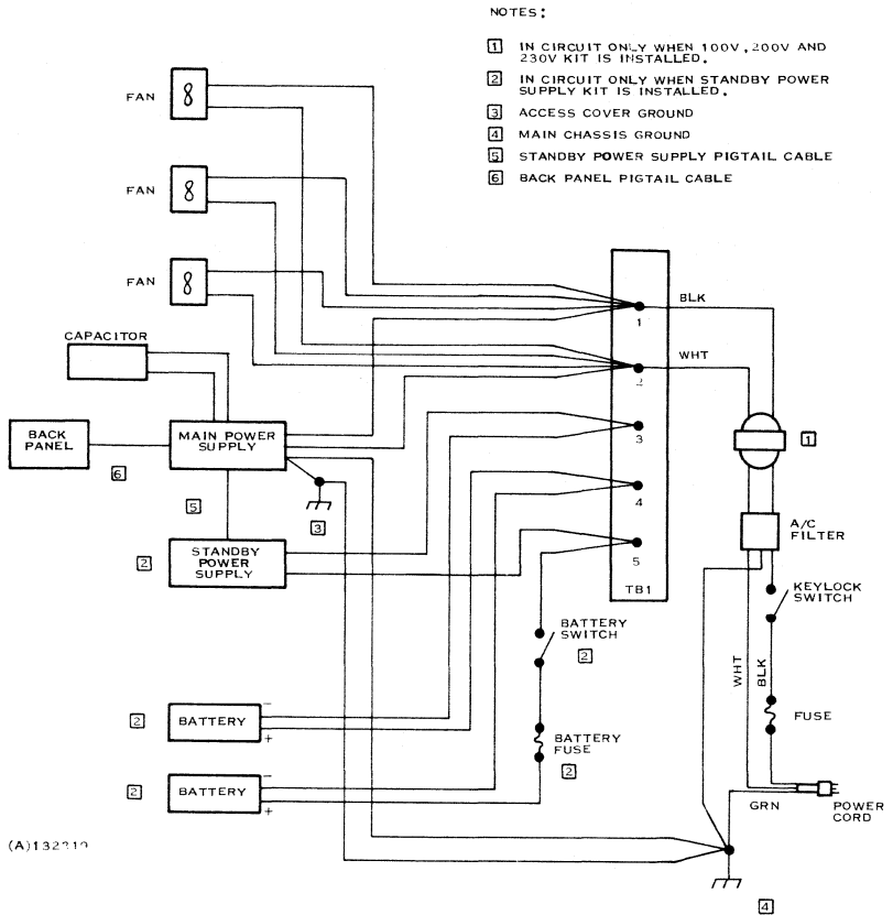
Figure G-1. Chassis Wiring for 6-Slot or 13-Slot Chassis
